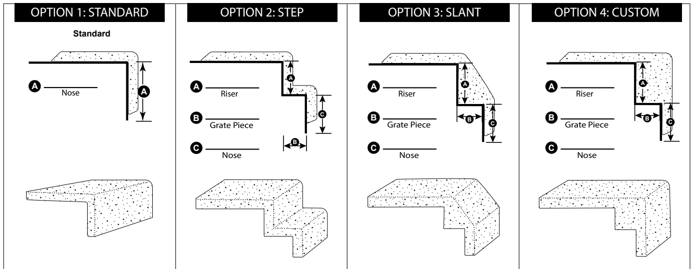
Side Views
